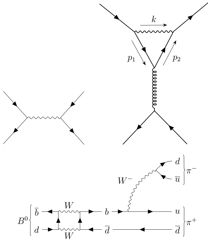
Figure 1: Using tikz-feynmann
