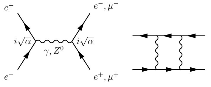
Figure 2: Using feynmp
