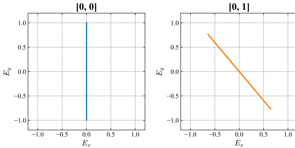
Figure 1: Left panel: V = 0 , Q < 0 , U = 0 , i.e., \pi/2 linear polarization, right panel: V = 0 , Q = 0 , U < 0 , i.e., 3\pi/4 linear polarization.
