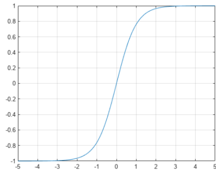
(b) Tanh activation function
