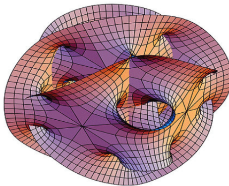
Figure 1: An example of a Calabi yau Manifold
