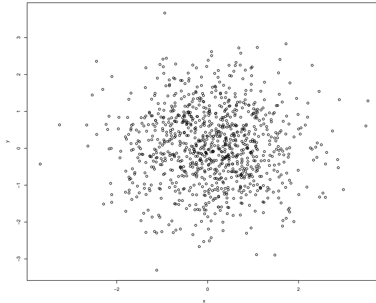
Figure 1: Scatter plot of x and y.
